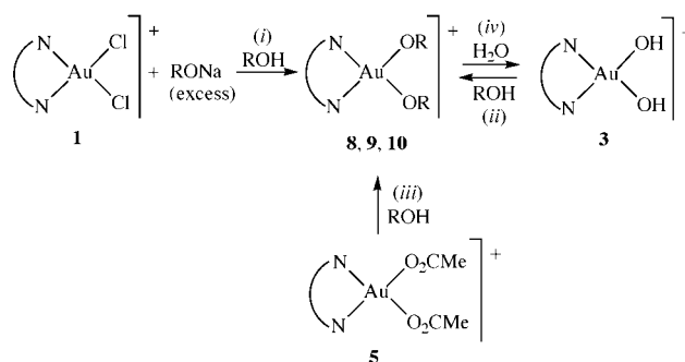
Scheme 2 (i) R = Me or Et; (ii) R = Me or Et; (iii) R = Me, Et or Pr i . R = Me 8 ; Et 9 or Pr i 10 .
