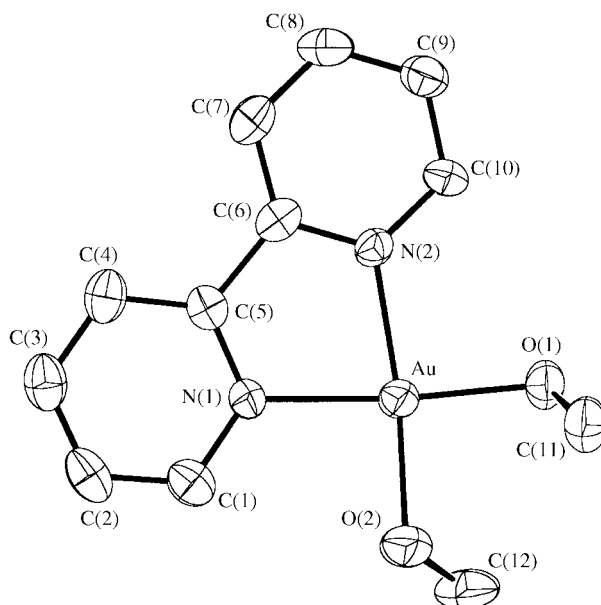
Fig. 1 An ORTEP view of the [Au(bpy)(OMe) 2 ] + cation in compound 8 . Thermal ellipsoids are drawn at the 30% probability level.
